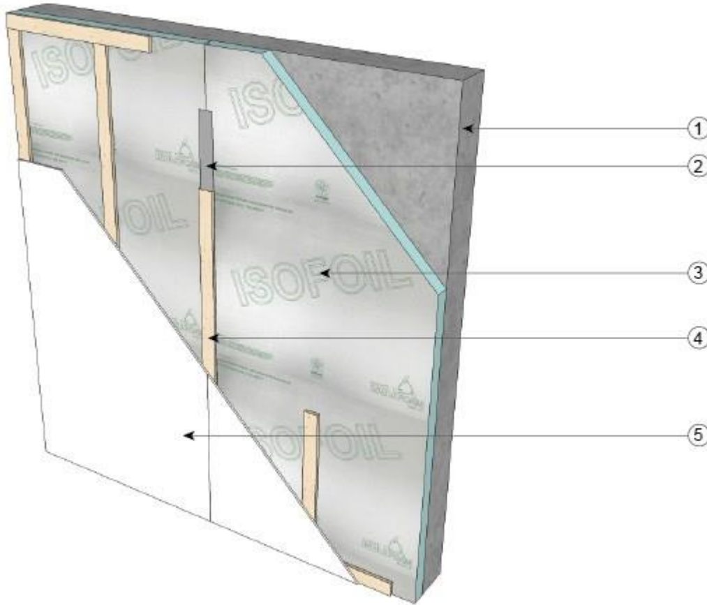
Figure 1. “Isofoil, PROfoil, EZfoil” adjacent to the furred air space assembly installed within the manufacturer’s designated wall assembly No. 1:
