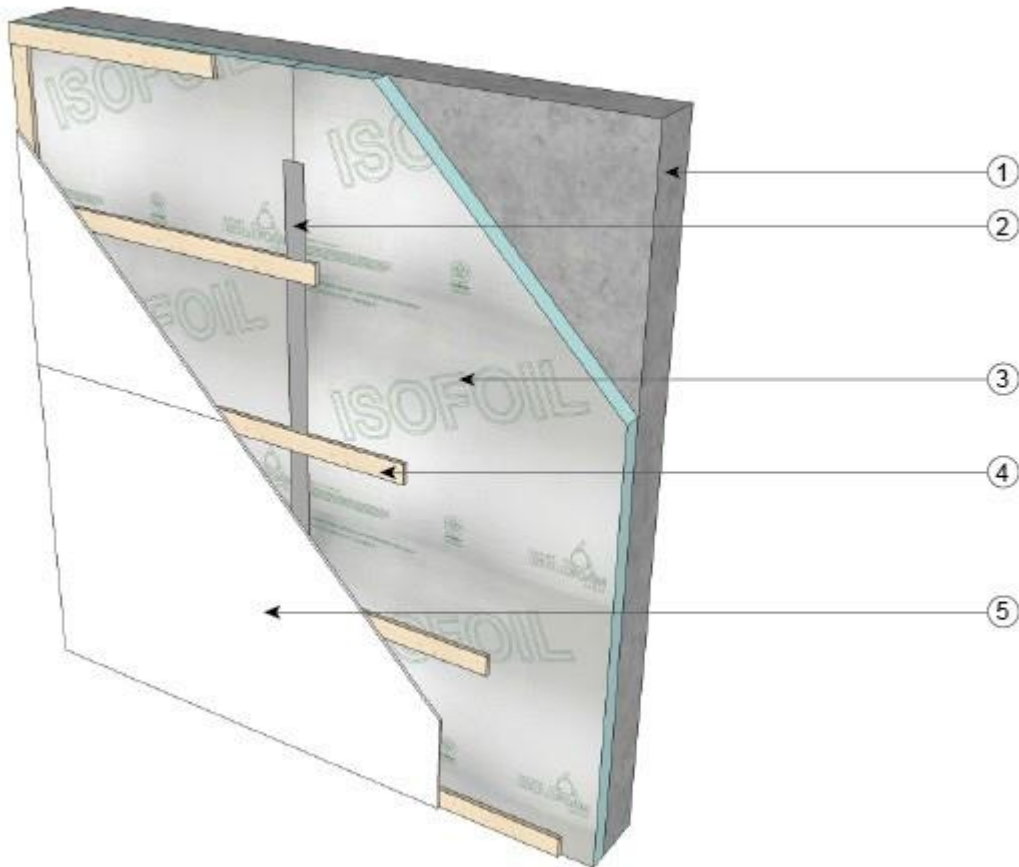
Figure 2. “Isofoil, PROfoil, EZfoil” adjacent to the furred air space assembly installed within the manufacturer’s designated wall assembly No. 2:
