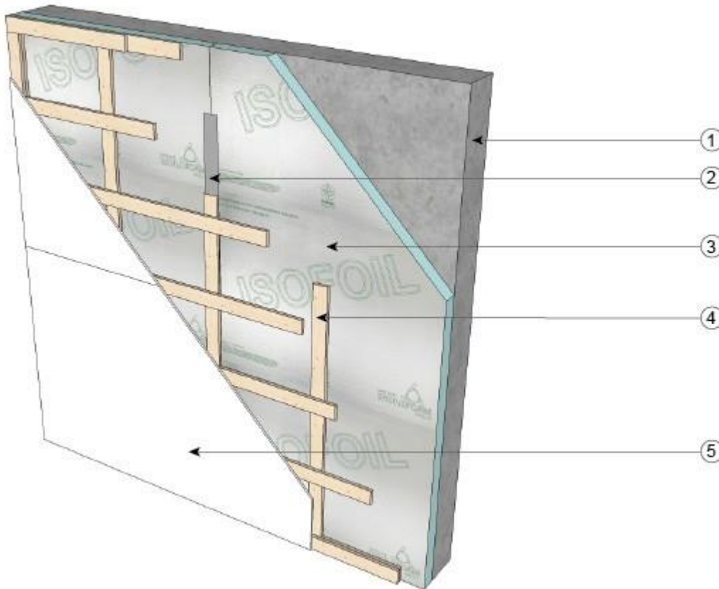
Figure 5. “Isofoil, PROfoil, EZfoil” adjacent to the furred air space assembly installed within the manufacturer’s designated wall assembly No. 5:
