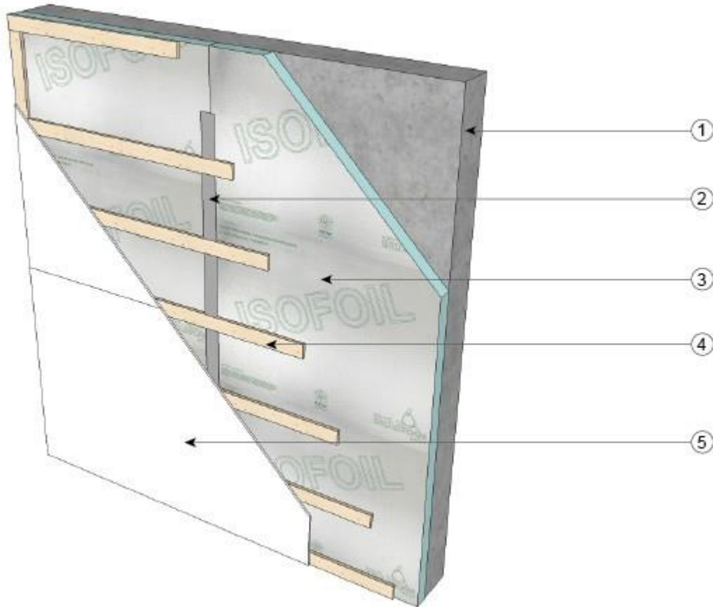
Figure 3. “Isofoil, PROfoil, EZfoil” adjacent to the furred air space assembly installed within the manufacturer’s designated wall assembly No. 3:
