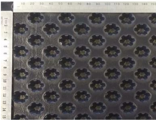
Figure 1. Side facing soil
